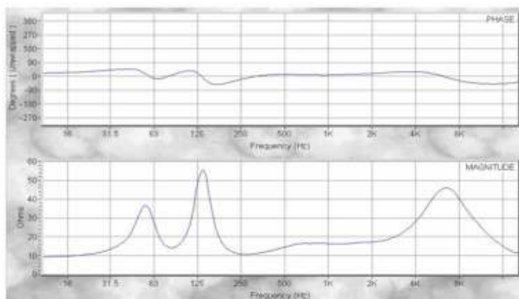
Bodeplot impedance: phase and amplitude
