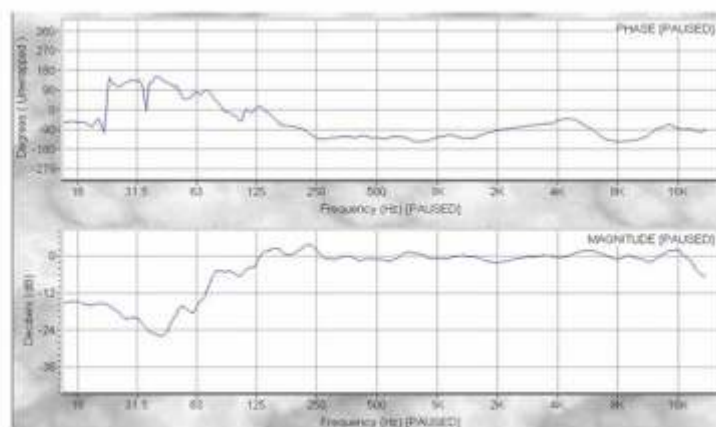
Bodeplot frequency response: phase and amplitude
